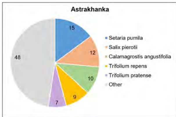
S3 Pie charts of proportions (%) of the five dominant (colored sectors) and the rest of the species (grey sector) at the sites
