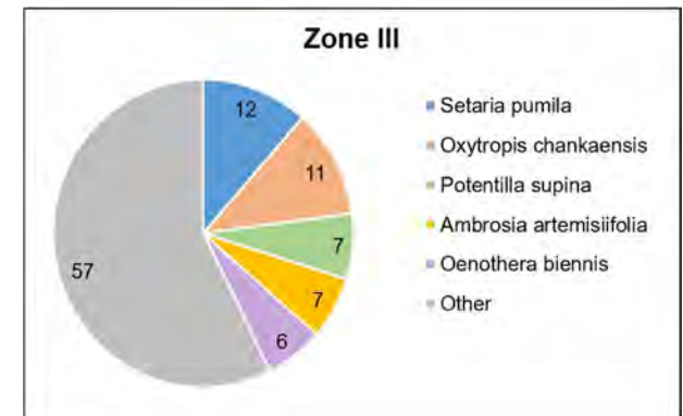
S5 Pie charts of proportions (%) of the five dominant species (colored sectors) and the rest of the species (grey sector) in the zones
