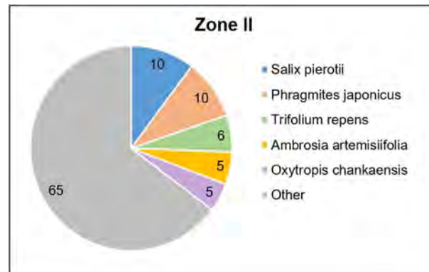
S5 Pie charts of proportions (%) of the five dominant species (colored sectors) and the rest of the species (grey sector) in the zones
