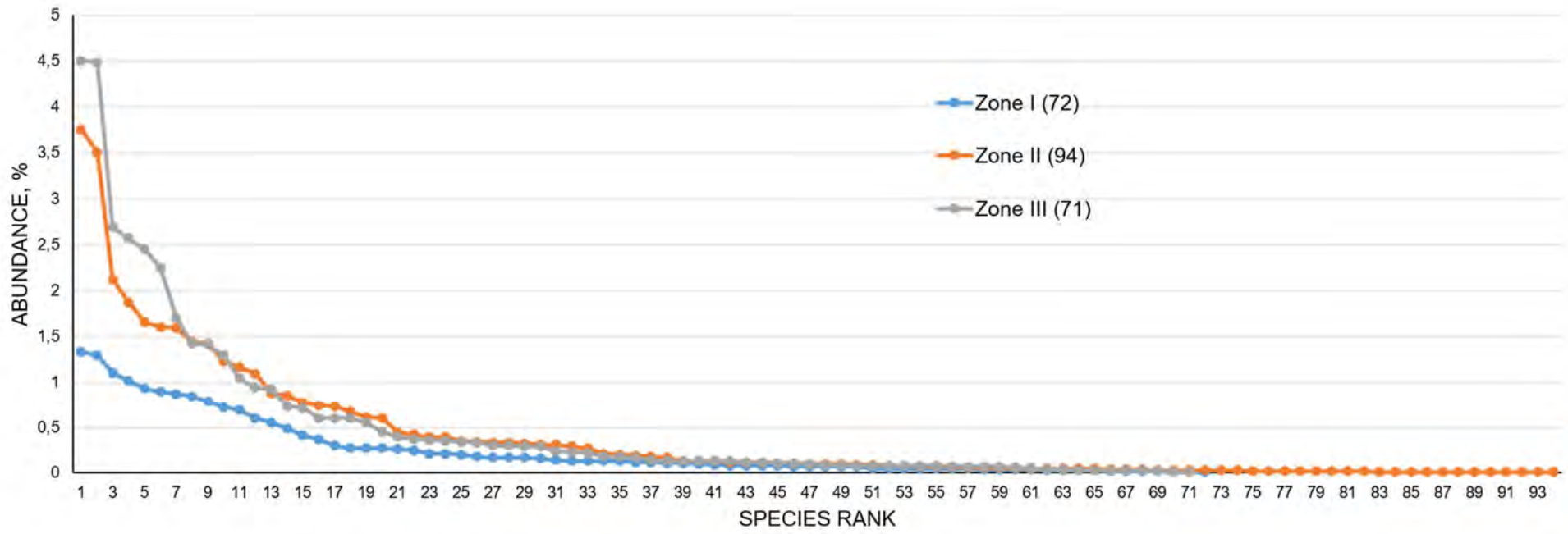
S4 Curves of species dominance in the zones.
