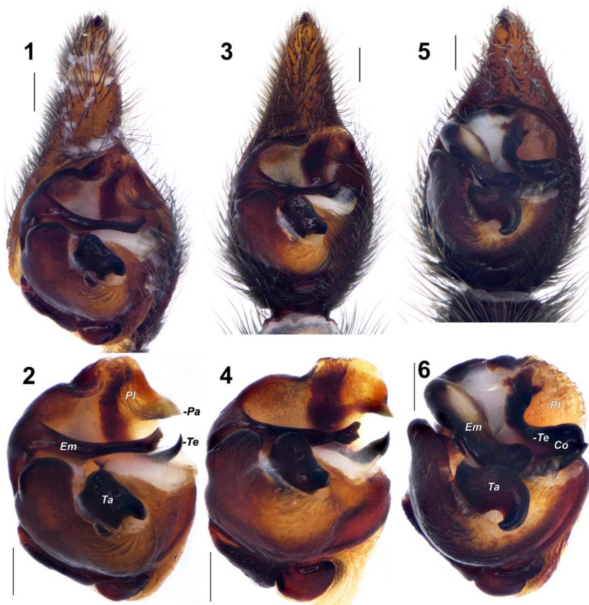
Figs 1–6. Bulbus of Acantholycosa irinae sp.n. (1–2), A. marusiki sp.n., (3–4) and Sibirosica arsenyevi sp.n. (5–6): 1, 3, 5 — palp, ventral view; 2, 4, 6 — bulb, ventral view. Scale: 0.2 mm. Abbreviations: Em — embolus, Co — conductor, Pa — paleal apophysis, Pl — palea, Ta — tegular apophysis, Te — terminal apophysis.
