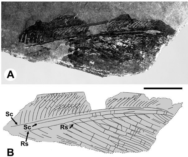
Figure 24 Polystoechotites sp. B, specimen SFU, Q-0094; apical portions of overlapping fore-wings. A , photograph of part; B , combined drawing of part and counterpart. For abbreviations see Materials and Methods. Both to scale; scale bar = 5 mm.
