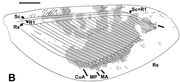
Figure 15 Palaeopsyrops maculatus Andersen, holotype, GMUC, Danekræ No. 298; hind-wing. A , photograph; B , drawing. For abbreviations see Materials and Methods. Both to scale; scale bar = 5 mm.
