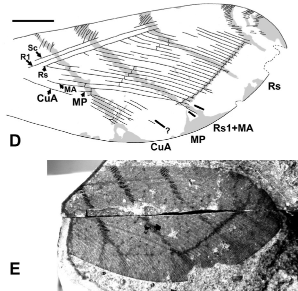
Figure 10 Palaeopsychoptera angustifasciatus Andersen, fore-wings. A , photograph of holotype, GMUC, Danekræ No. 89; B , photograph of paratype 2, GMUC, MGUH27522; C , photograph of GMUC specimen MGUH27524; D , drawing of holotype; E , photograph of paratype 9, GMUC, MGUH27523. For abbreviations see Materials and Methods. All approximately to scale; scale bar = 5 mm.
