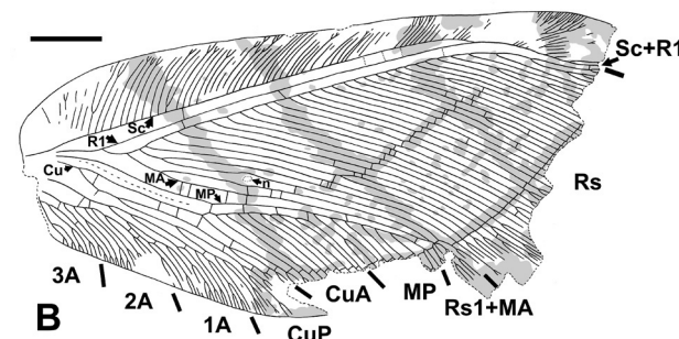
Figure 11 Palaeopsyrops quadratus sp. nov., holotype, GZG, GZG 001261/1a/1b; fore-wing. A , photograph of part; B , drawing from part and counterpart. For abbreviations see Materials and Methods. Both to scale; scale bar = 5 mm.
