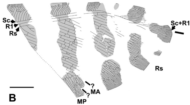
Figure 13 Palaeopsyrops maringerae sp. nov., holotype, SR, SR97-08-05; fore-wing. A , photograph; B , drawing. For abbreviations see Materials and Methods. Both to scale; scale bar = 5 mm.
