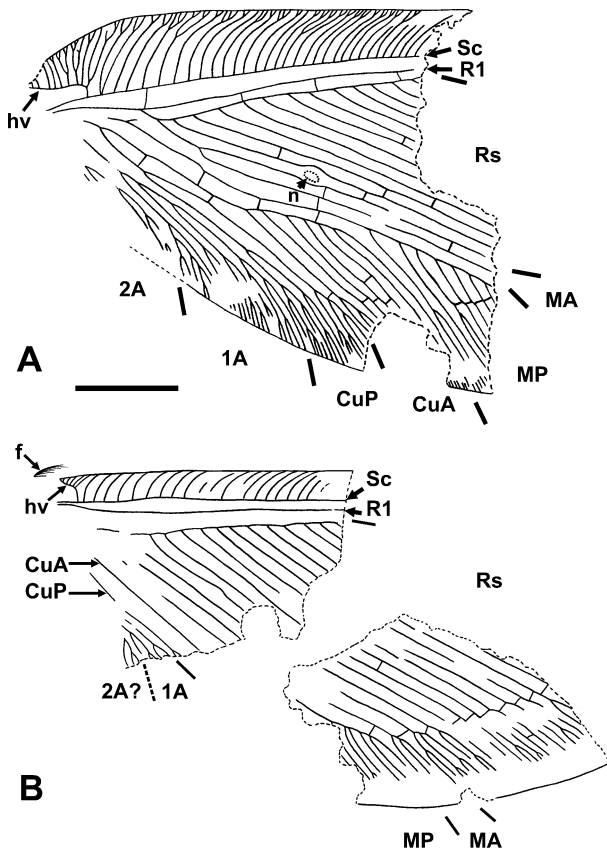
Figure 9 Palaeopsychoptera abruptus Andersen, paratype 1, GMUC, Danekræ No. 168. A , drawing of fore-wing; B , drawing of hind-wing. f , frenulum. For other abbreviations see Material and Methods. Both to scale; scale bar = 5 mm.
