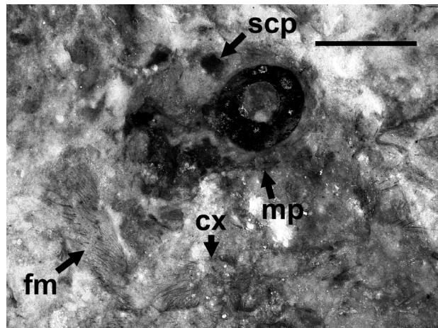
Figure 7 Anterior portion of body of Palaeopsychops abruptus , paratype 1, GMUC, Danekræ No. 168. cx, coxa; fm, femur; mp, maxillary palp; scp, scape. Scale bar = 2 mm.
