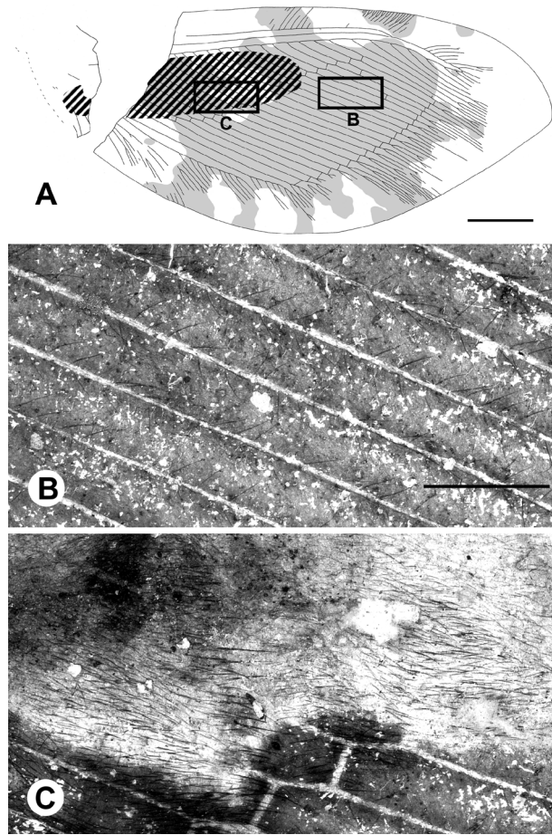
Figure 17 Dense macrotrichia across both membrane and veins in a region of the hind-wing of Palaeopsychops setosus (holotype, part). A , crosshatching, marks region of pilosity; ‘B’, location of enlarged area shown in Fig. 17B; ‘C’, location of enlarged area shown in Fig. 17C. Scale bar = 5 mm; B , close-up in region of normal long macrotrichia on veins, not membrane; C , close-up of densely pilose region showing macrotrichia across both light and dark coloured wing areas. B and C both to scale; scale bar = 1 mm.
