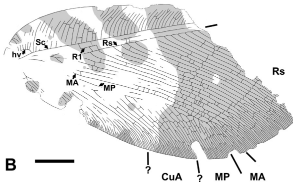
Figure 14 Palaeopsyrops timmi sp. nov., holotype, SR, SR02-25-01; fore-wing. A , photograph; B , drawing. For abbreviations see Materials and Methods. Both to scale; scale bar = 5 mm.
