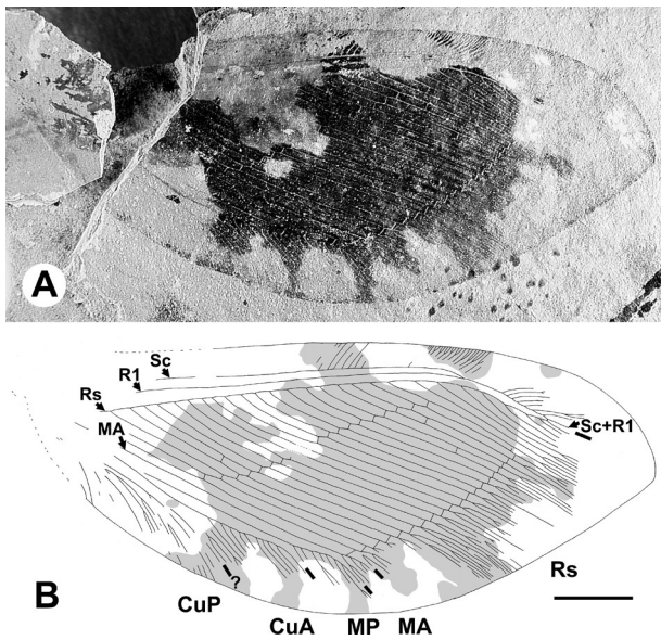
Figure 16 Palaeopsychops setosus sp. nov., holotype, UA, UAFIC8354 (part) and UAFIC8335 (counterpart); hind-wing. A , photograph of part; B , combined drawing from part and counterpart. For abbreviations see Materials and Methods. Both to scale; scale bar = 5 mm.
