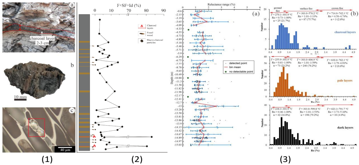
Fig. 1. (a) Charcoal layers, (b) charcoal particles, and (c) inertinite preserved in the Jinsuo lignite seam.
